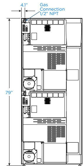
BACK VIEW - Gas
