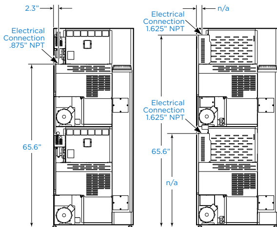
Electrical Connections - Gas Models
