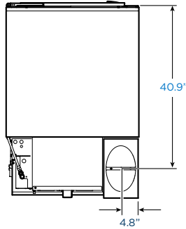
Exhaust Outlet Locations - All Heating Types
