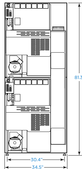
BACK VIEW
