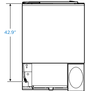
TOP VIEW - Gas
